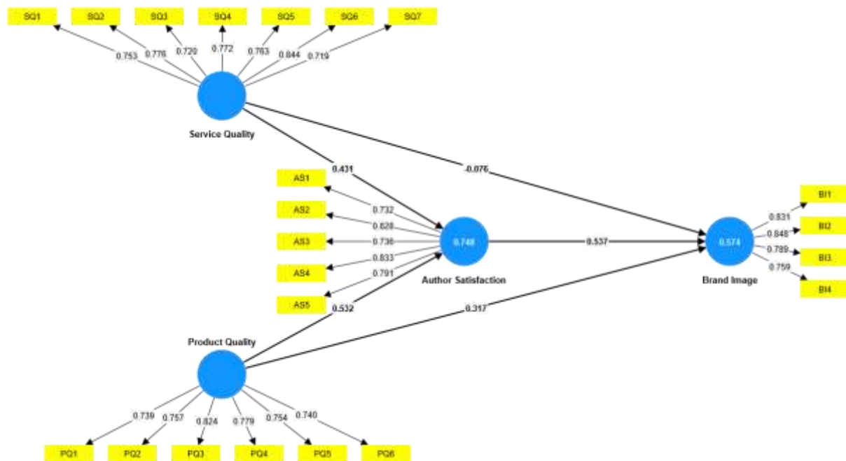
Gambar 3. Output Inner Model
