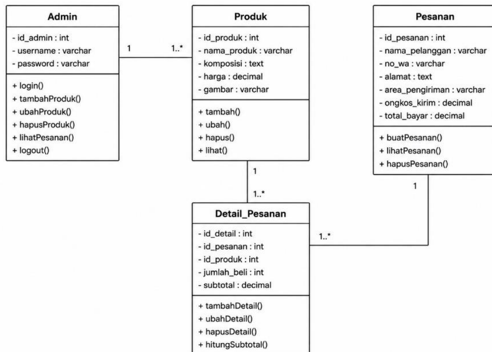
Gambar 3. Class Diagram
