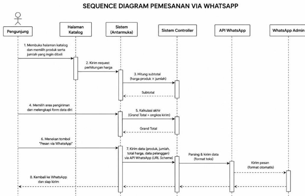
Gambar 4. Sequence Diagram Alur
