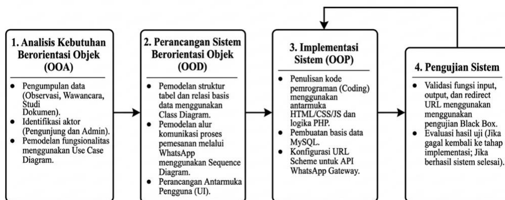
Gambar 1. Metode Waterfall
