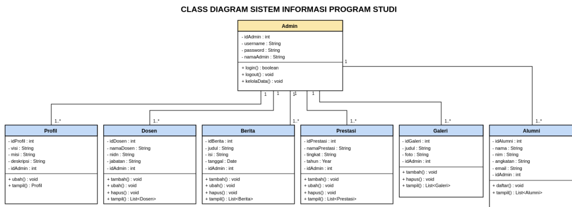
Gambar 3. Class Diagram Sistem
