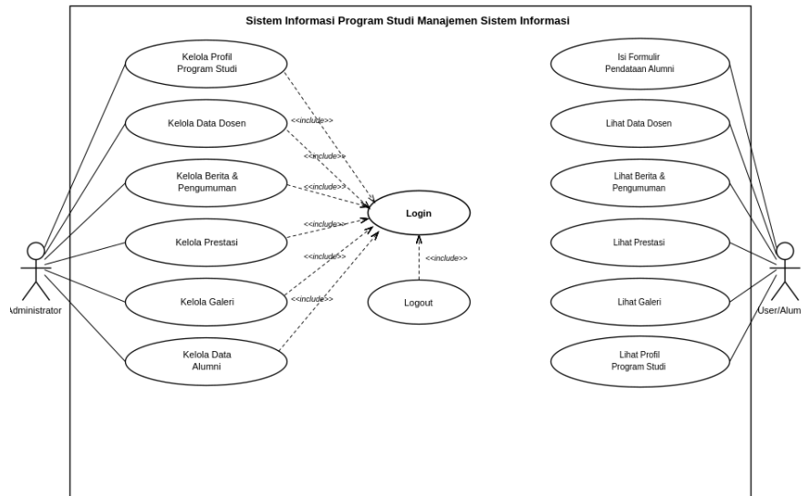
Gambar 2. Use Case Diagram Sistem
