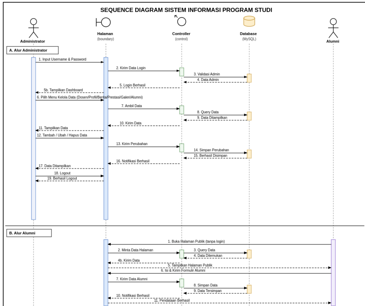
Gambar 4. Sequence Diagram Sistem Informasi Program Studi
